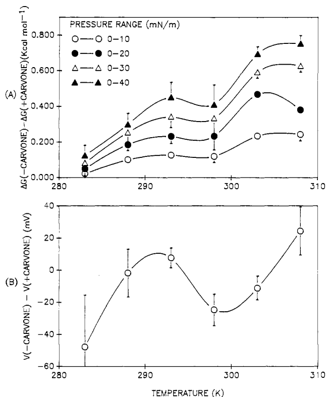
Figure 2. Differences in free energy of compression ( \Delta G ) and surface potential ( \Delta V ) between L-DPPC monolayers made on subphase containing 5 mM (-) and (+)-carvone as functions of temperature. Differences in free energy (A) calculated 3 for indicated pressure ranges; differences in surface potential (B) measured 3 for fully compressed monolayers. Points represent mean values of experimental data ( \pm SD) while curves are cubic spline interpolations.
